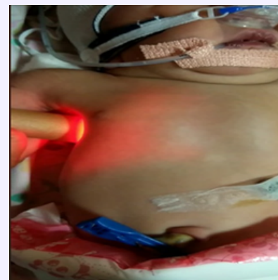
Figure 6.2 Transillumination
