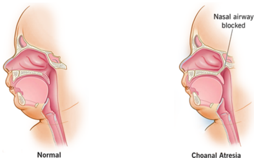
Figure 6.7 Choanal Atresia
