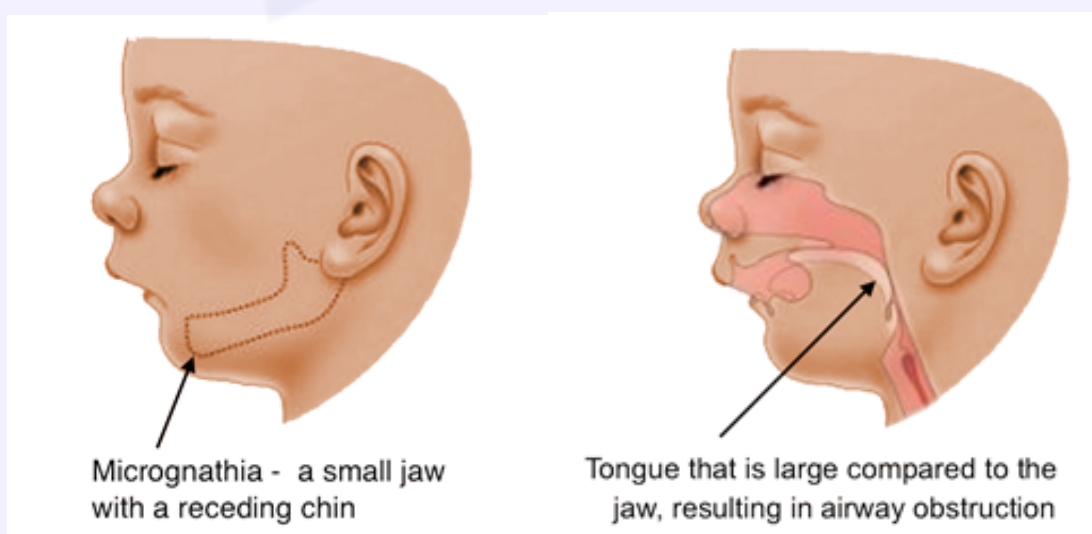
Figure 6.8 Robin Sequence
